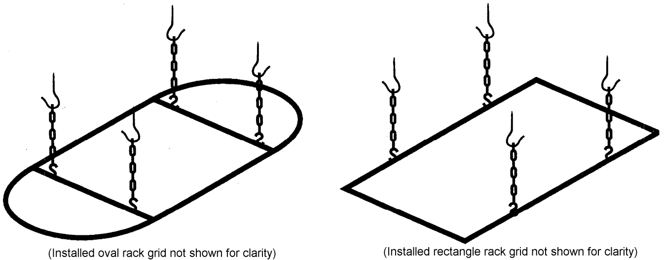
Figure 2 Hook and Chain Assembly
